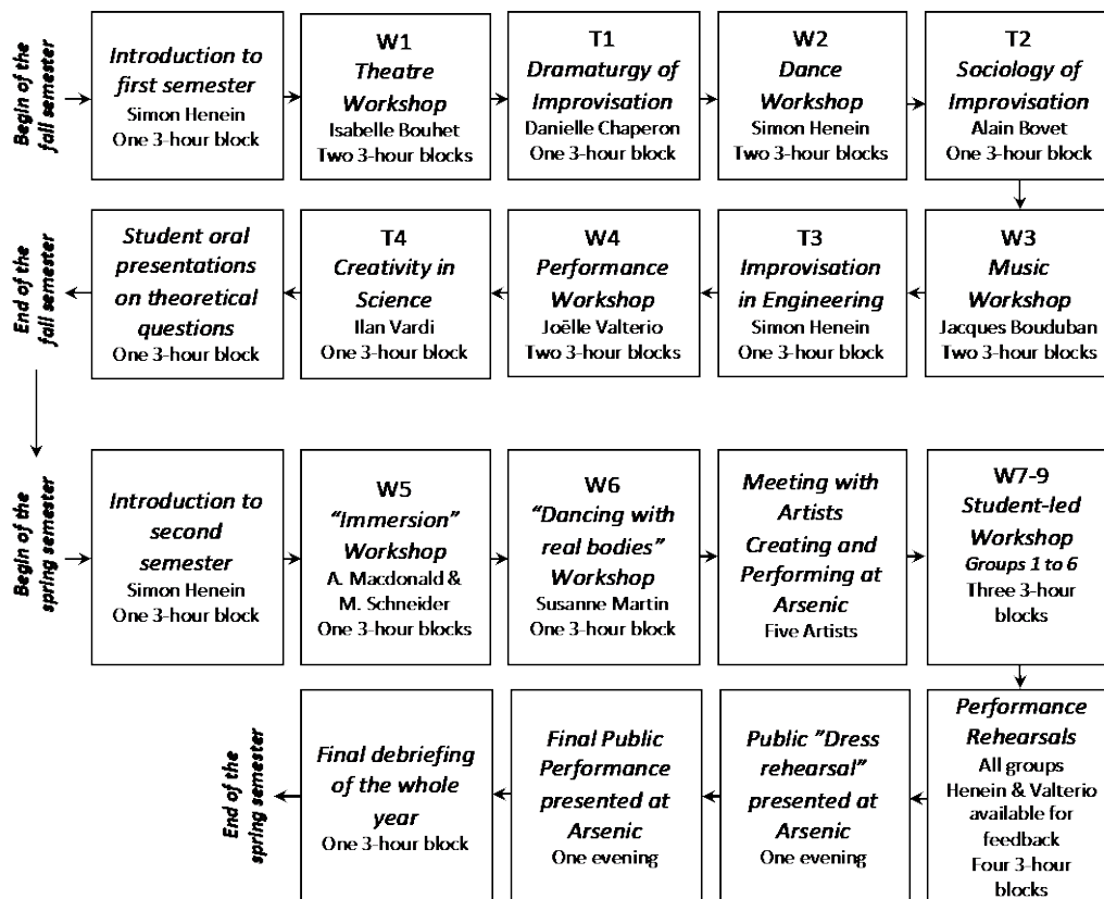
Fig. 1: Structure of the Improengineering course, consisting of twenty-eight 3-hour weekly blocks spread over two 14-week semesters.
